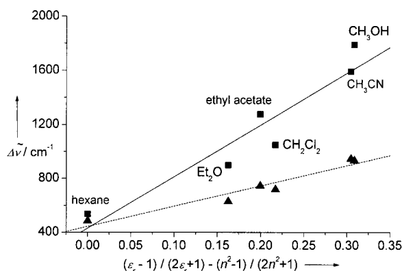
Figure 4. Correlation of the Stokes Shift between the absorption and emission maxima \Delta\tilde{\nu} = \Delta\tilde{\nu}_{\text{abs}} - \Delta\tilde{\nu}_{\text{em}} and the Lippert–Mataga polarity parameter of the solvent for dyes 5a (■) and 7 (▲).
