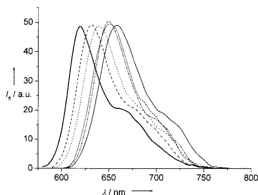
Figure 3. Fluorescence spectra of dye 7 for solvents of increasing polarity. From left to right: (—, thick) n -hexane, (---) diethyl ether, (••••) ethyl acetate, (—•—•) dichloromethane, (short dashes) acetonitrile, (—, thin) methanol.
