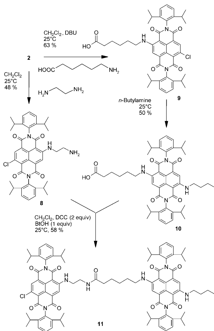
Scheme 3. Synthesis of bichromophoric compound 11 .
