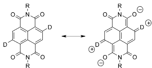
Scheme 2. Resonance model for dyes 3–7 which explains the strong impact of electron donor substituents D on the absorption and emission wavelengths as well as the significant positive solvatochromism.
