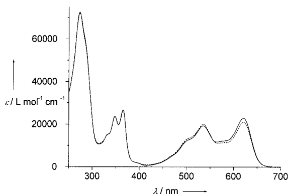
Figure 7. Absorption spectra of a 1.5 \times 10^{-5} M solution of dye 11 (solid line) and of a mixture of dyes 5a and 7 at the same concentration (dotted line) in dichloromethane.
