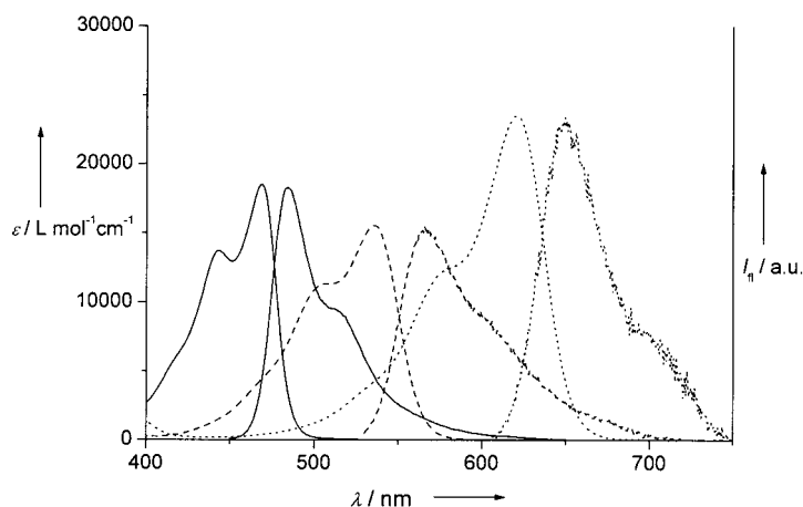
Figure 2. Absorption and fluorescence spectra of dyes 4 (solid line), 6 (dashed line) and 7 (dotted line) in dichloromethane.
