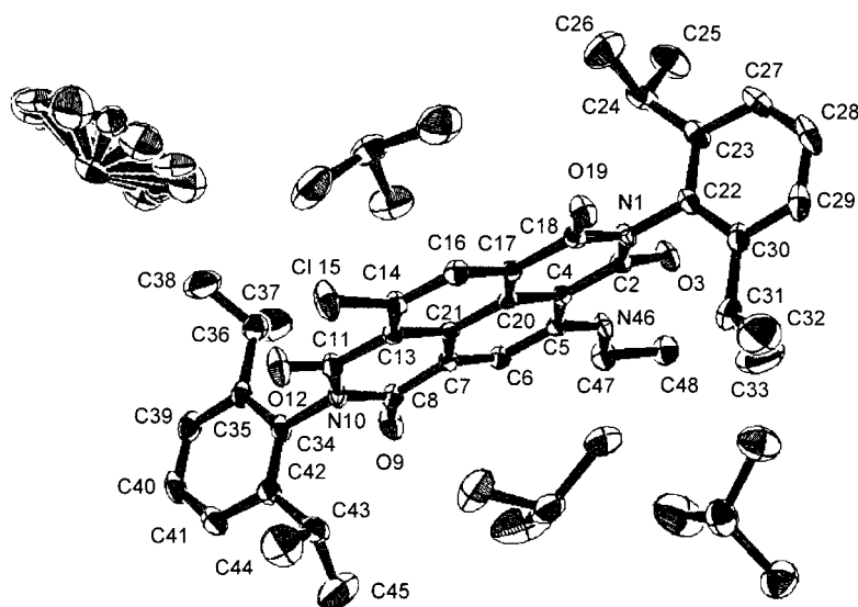
Figure 6. Structure of 5a (ORTEP plot) in the crystal showing the presence of four molecules of chloroform (one of them disordered) that fill the space created by the orthogonal connection ( \theta = 83^\circ ) of the naphthalene bisimide and the diisopropylphenyl substituents.
