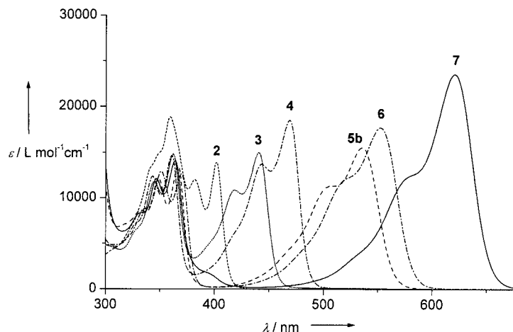
Figure 1. UV/Vis absorption spectra of dyes 2–7 in dichloromethane.
