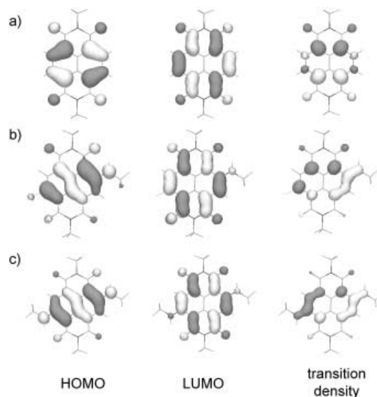
Figure 5. HOMO, LUMO, and transition density for a) N,N' -dimethylnaphthalene 1,4,5,8-tetracarboxylic acid bisimide and its b) 2-chloro-6-dimethylamino- and c) 2,6-dimethylamino-substituted derivatives according to CNDO/S calculations of AM1 optimized molecules.
