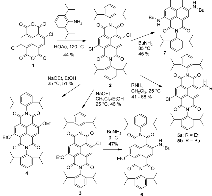
Scheme 1. Synthesis of naphthalene bisimide dyes 3–7 .
