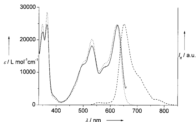
Figure 8. Absorption (dotted line), excitation (solid line; fluorescence detection at 660 nm), and fluorescence (dashed line; excitation at 500 nm) spectra for dye 11 in dichloromethane.
